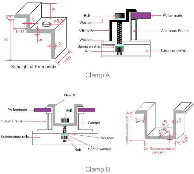
Figure 1 Mounting detail
