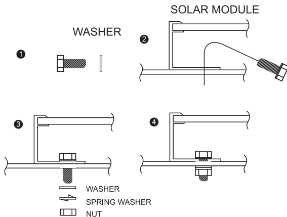
Figure 2 Mounting Details
